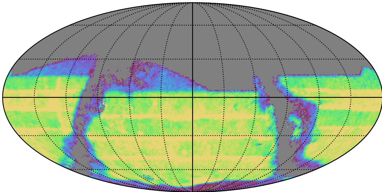
too_elab_r256_d2_giz_v3.4_10yrs : TDC_rate
