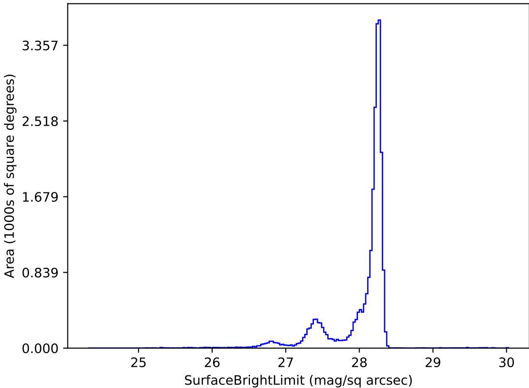
too_elab_r256_d2_giz_v3.4_10yrs y: SurfaceBrightLimit
