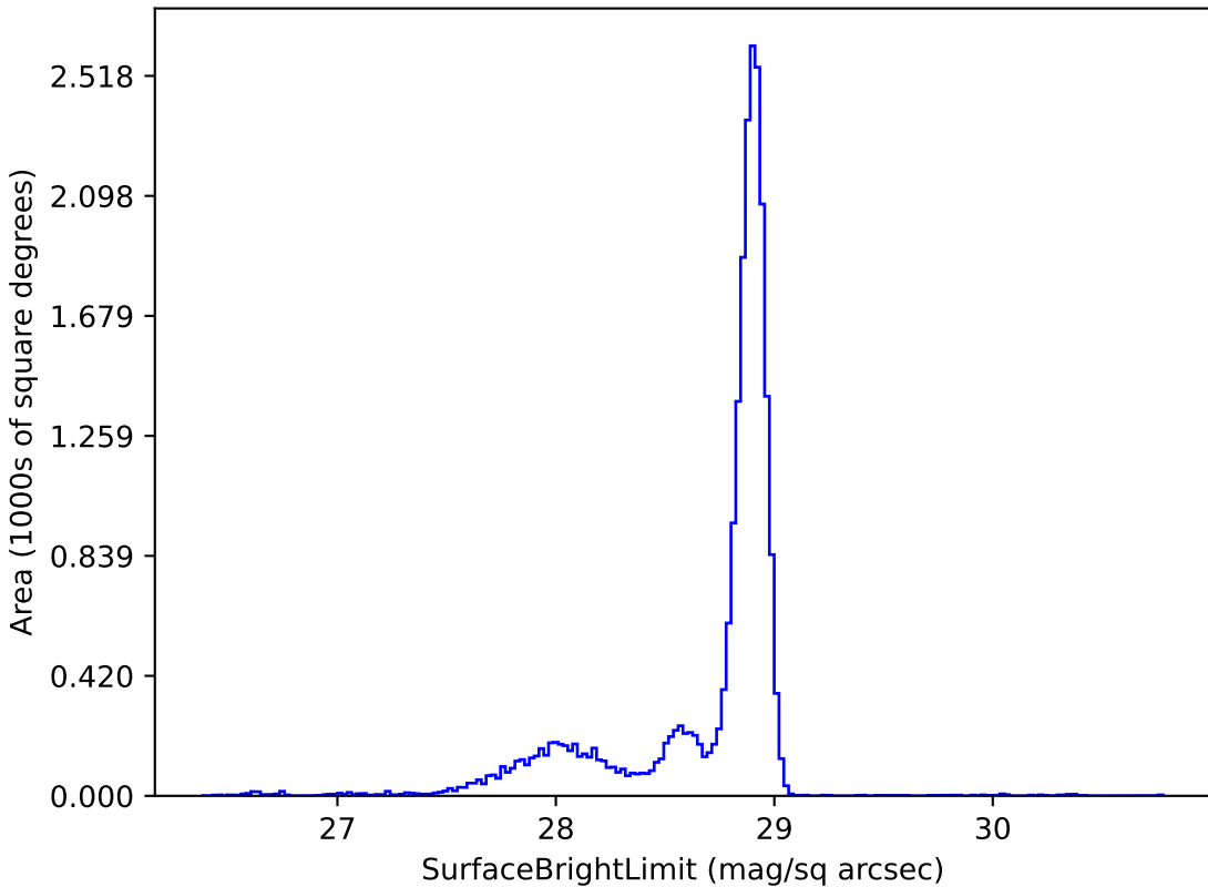
too_elab_r256_d2_giz_v3.4_10yrs u: SurfaceBrightLimit
