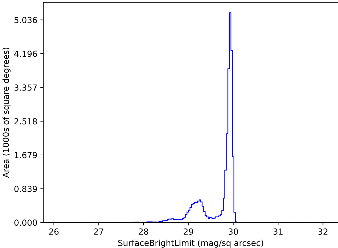
too_elab_r256_d2_giz_v3.4_10yrs i: SurfaceBrightLimit
