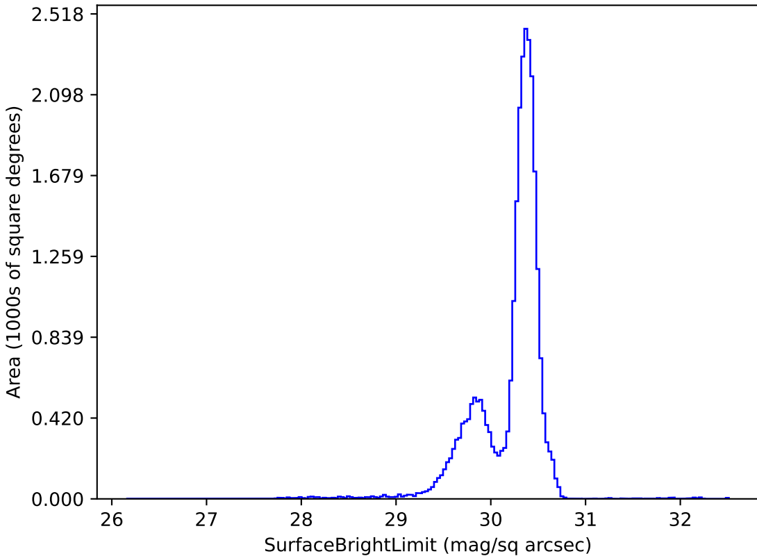
too_elab_r256_d2_giz_v3.4_10yrs g: SurfaceBrightLimit
