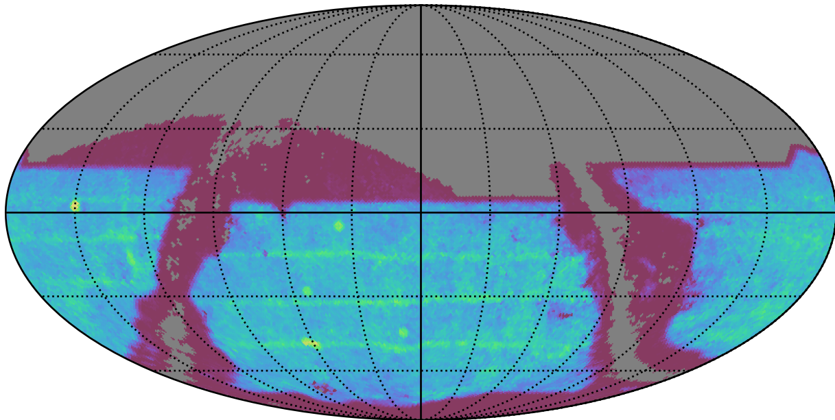
too_elab_r256_d2_giz_v3.4_10yrs : SNSLMetric
