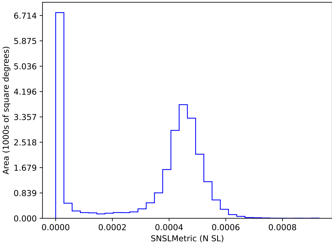
too_elab_r256_d2_giz_v3.4_10yrs : SNSLMetric
