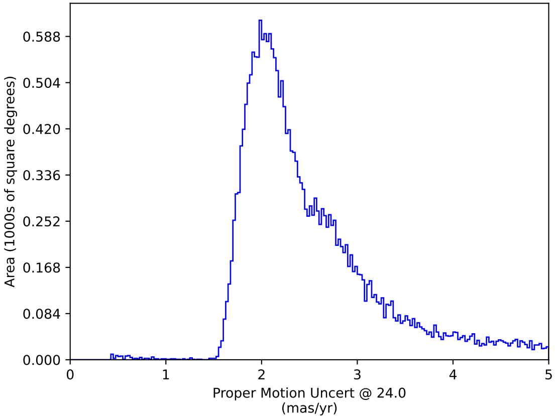
too_elab_r256_d2_giz_v3.4_10yrs : Proper Motion Uncert @ 24.0
