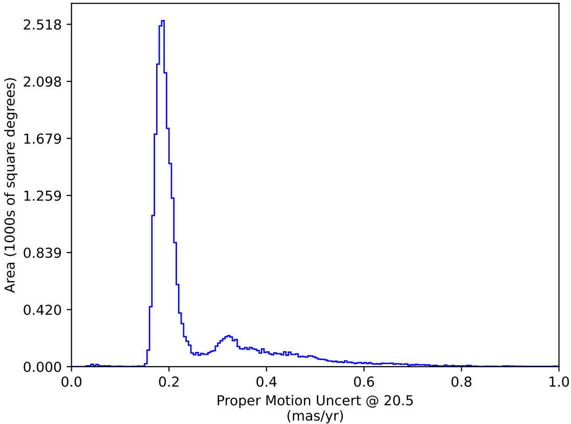
too_elab_r256_d2_giz_v3.4_10yrs : Proper Motion Uncert @ 20.5
