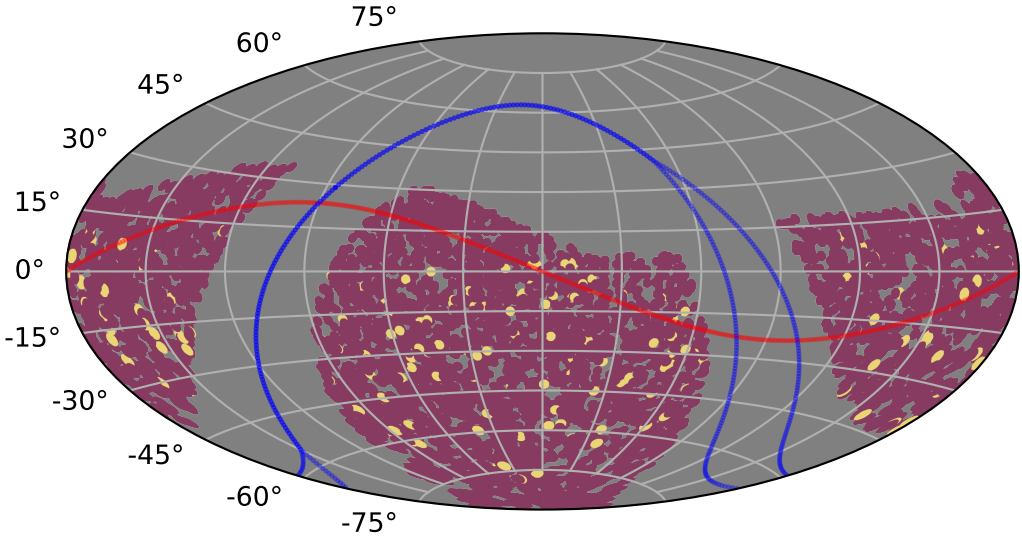
too_elab_r256_d2_giz_v3.4_10yrs : PrestoKNe_score_s
