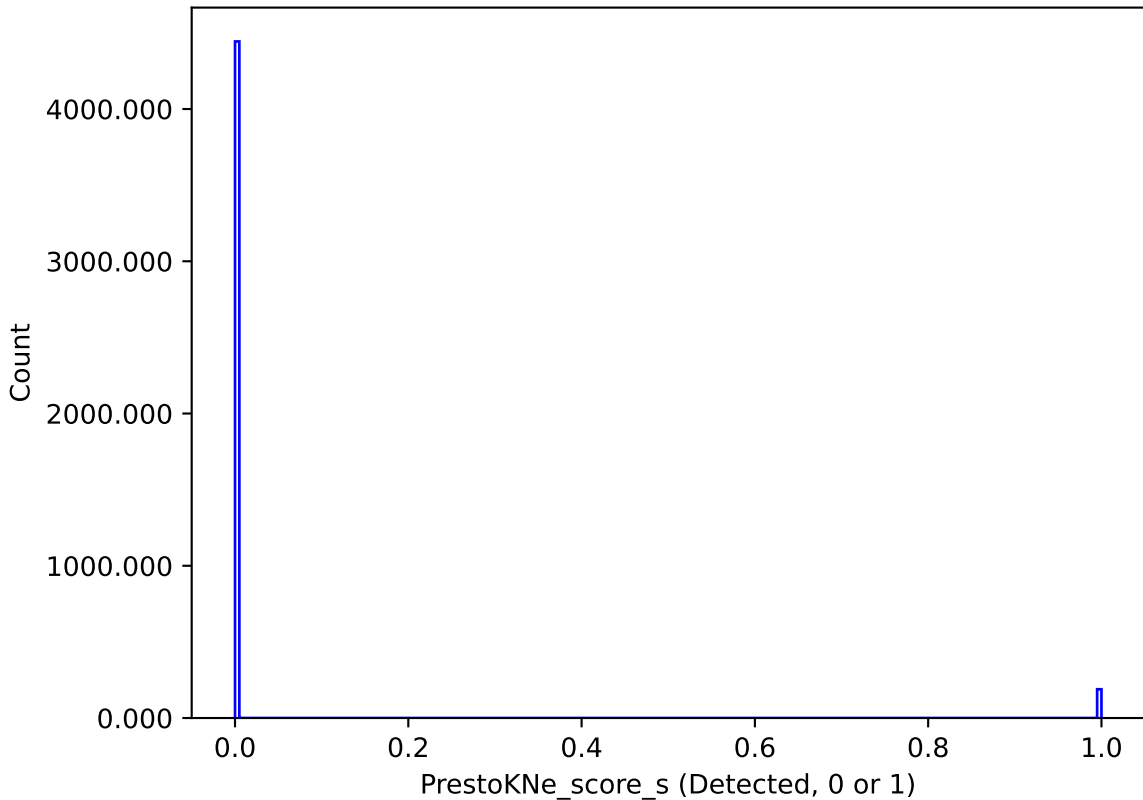
too_elab_r256_d2_giz_v3.4_10yrs : PrestoKNe_score_s
