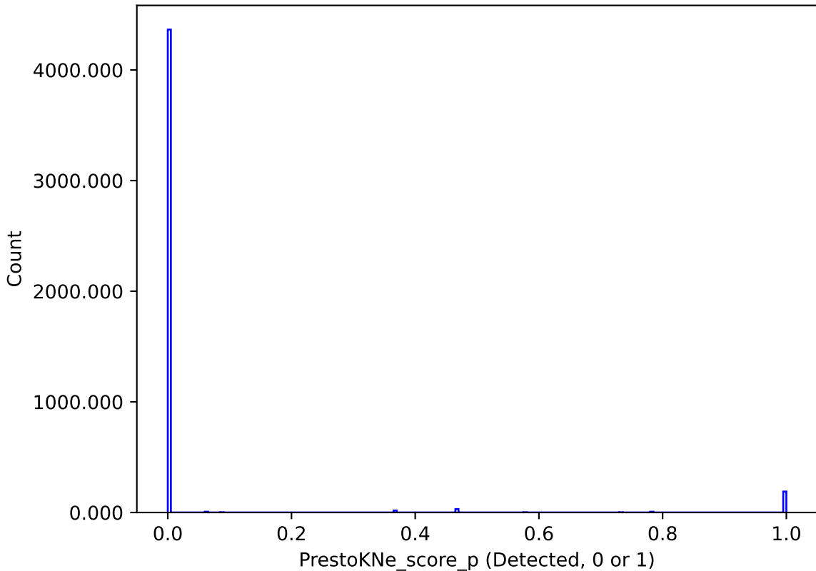
too_elab_r256_d2_giz_v3.4_10yrs : PrestoKNe_score_p
