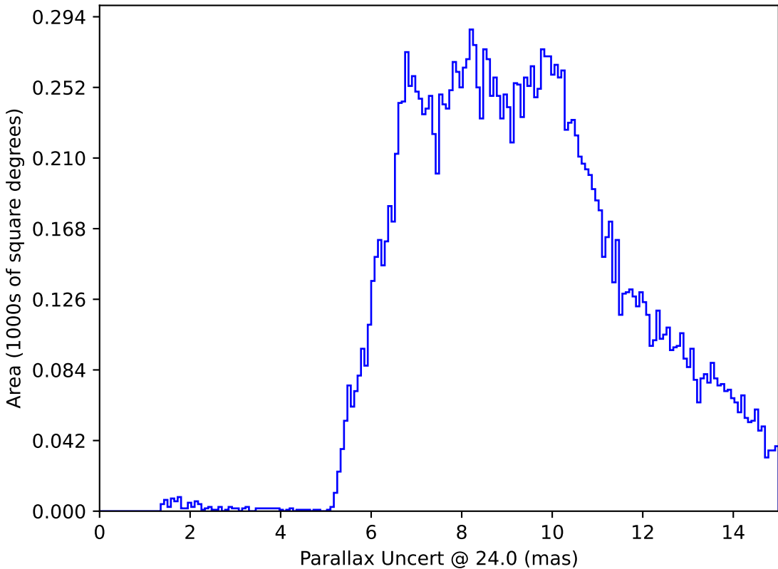
too_elab_r256_d2_giz_v3.4_10yrs : Parallax Uncert @ 24.0
