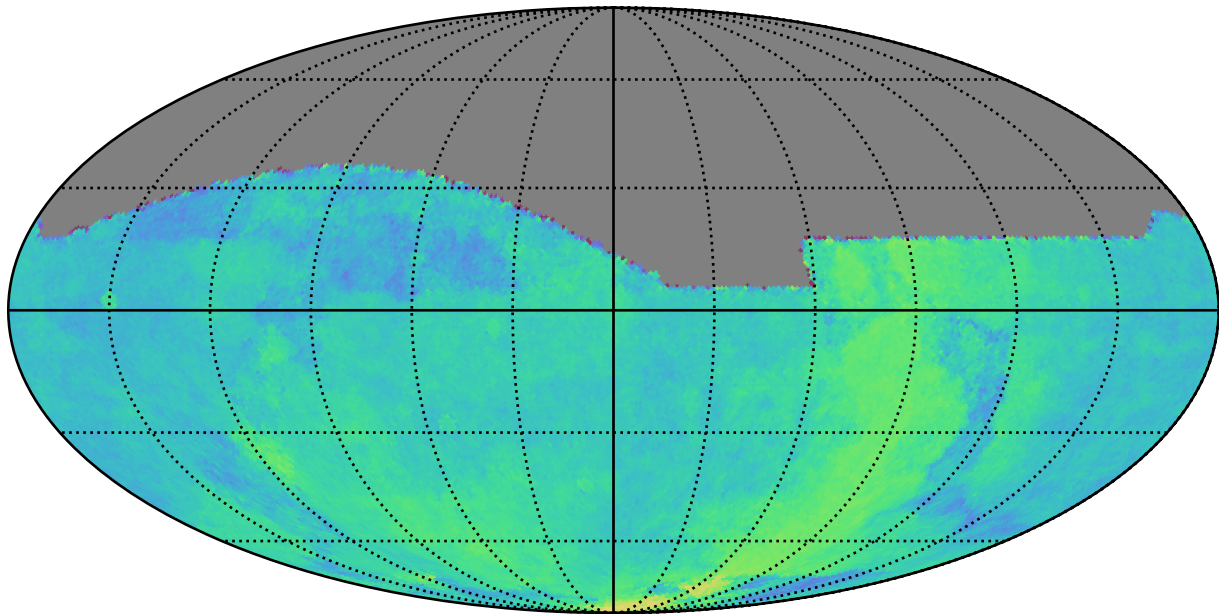
too_elab_r256_d2_giz_v3.4_10yrs : Parallax Coverage @ 24.0
