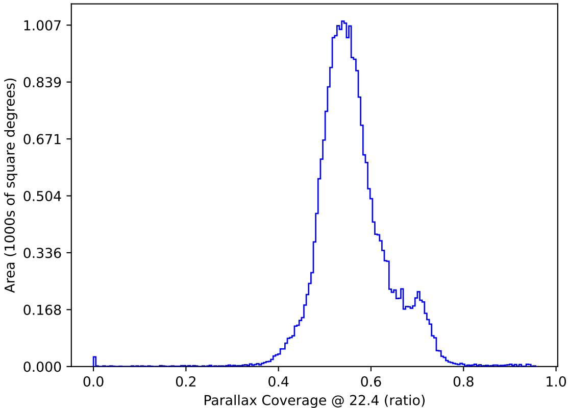
too_elab_r256_d2_giz_v3.4_10yrs : Parallax Coverage @ 22.4
