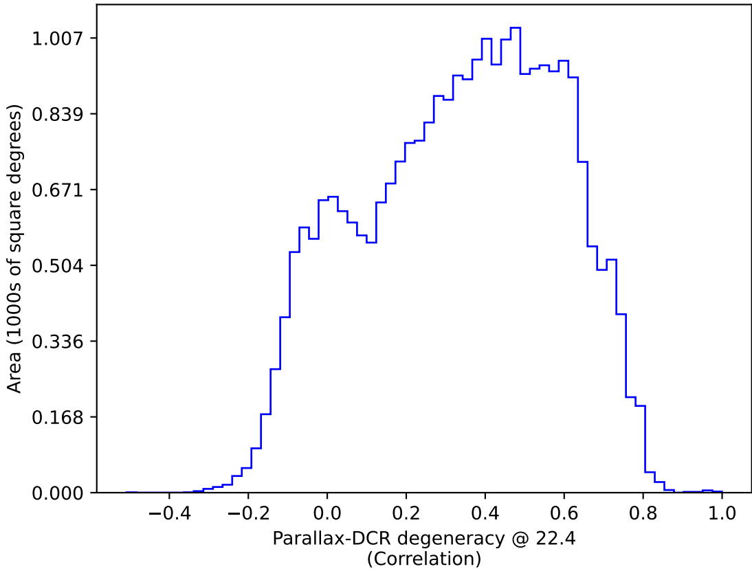
too_elab_r256_d2_giz_v3.4_10yrs : Parallax-DCR degeneracy @ 22.4
