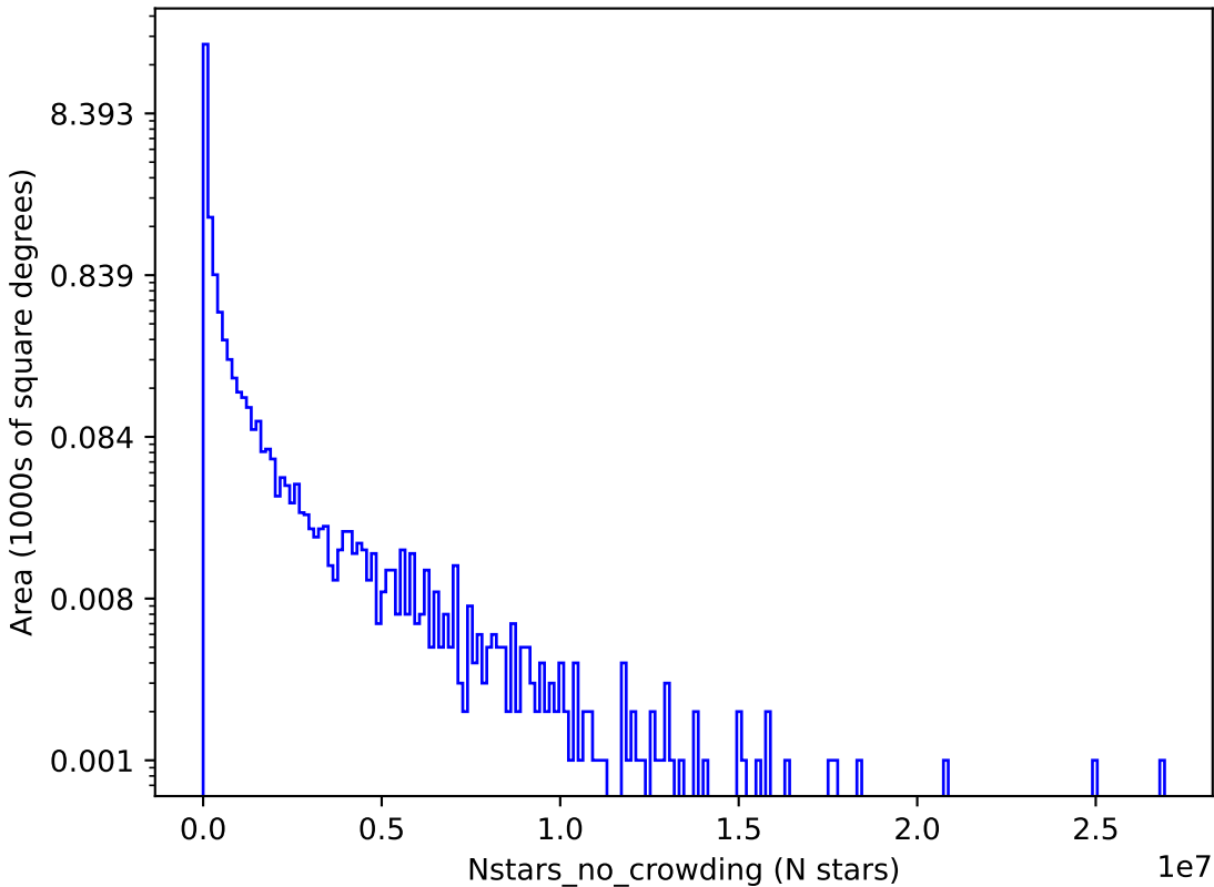
too_elab_r256_d2_giz_v3.4_10yrs i: Nstars_no_crowding
