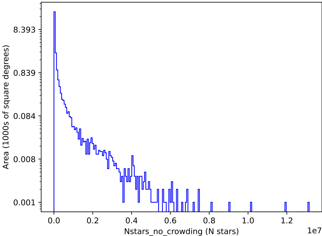
too_elab_r256_d2_giz_v3.4_10yrs g: Nstars_no_crowding
