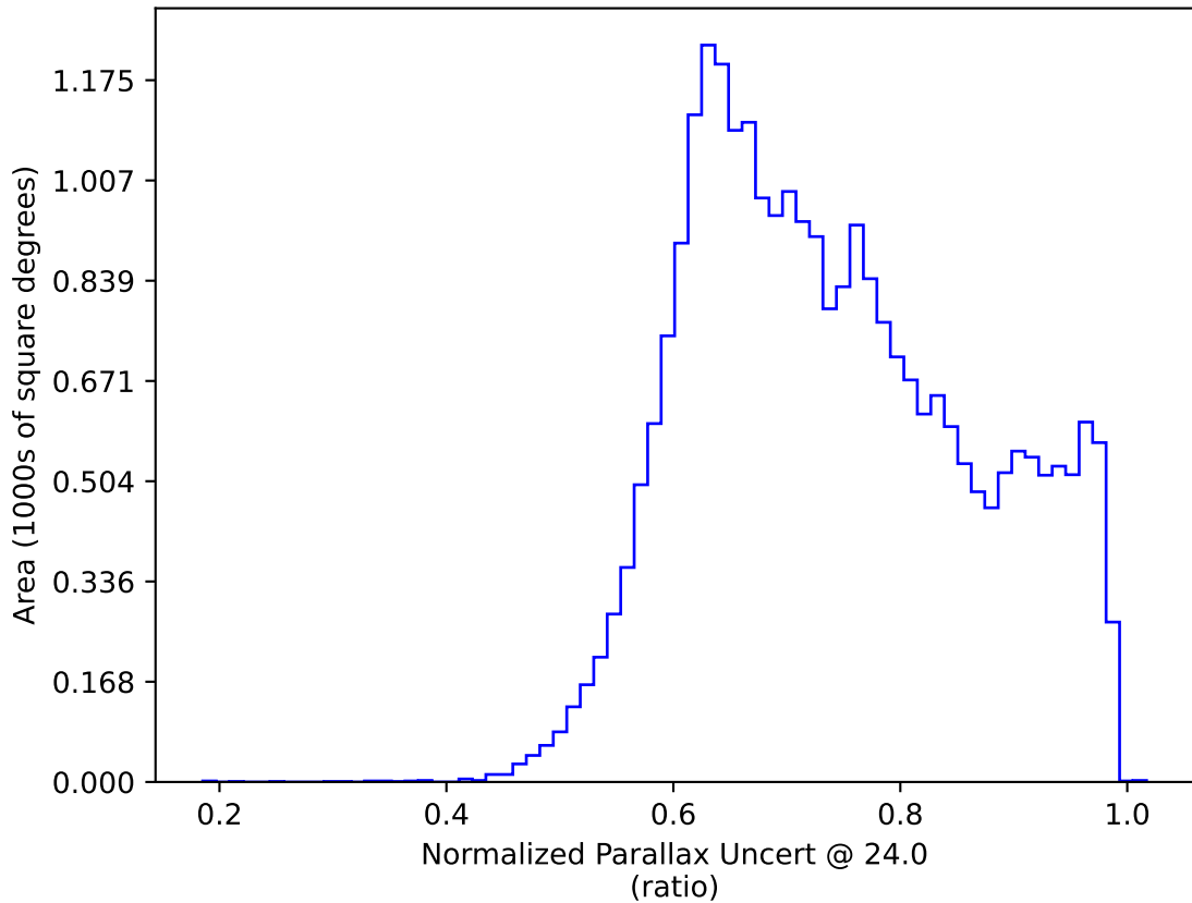
too_elab_r256_d2_giz_v3.4_10yrs : Normalized Parallax Uncert @ 24.0
