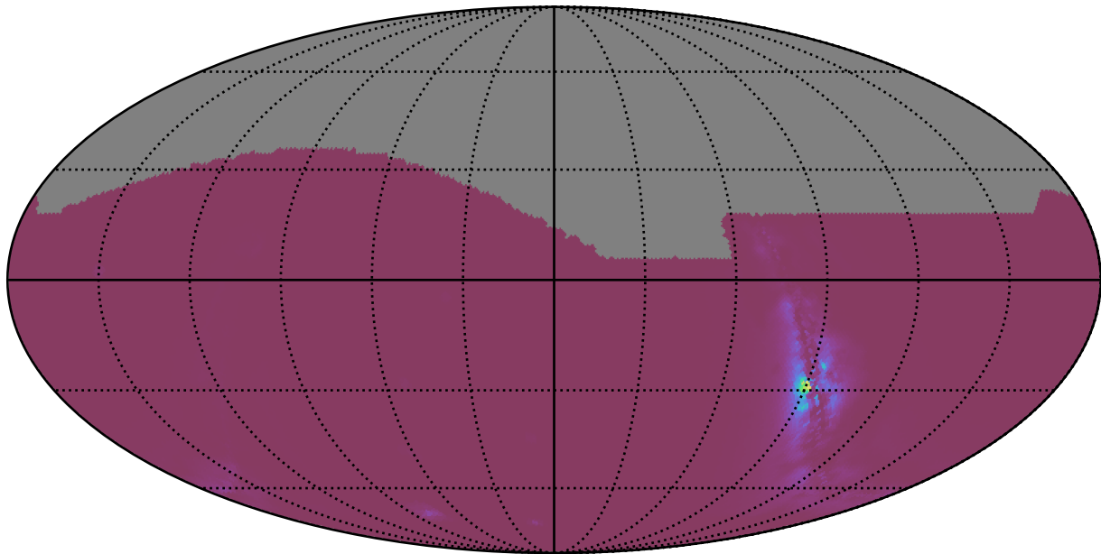
too_elab_r256_d2_giz_v3.4_10yrs : NlcPoints
