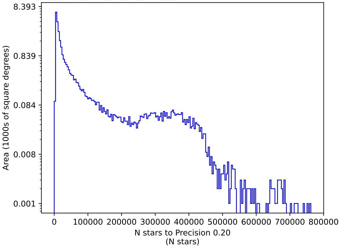
too_elab_r256_d2_giz_v3.4_10yrs g: N stars to Precision 0.20
