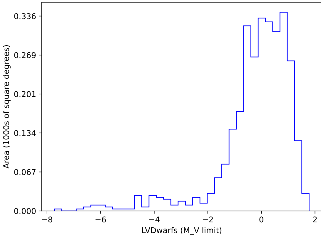
too_elab_r256_d2_giz_v3.4_10yrs gi SCP: LVDwarfs
