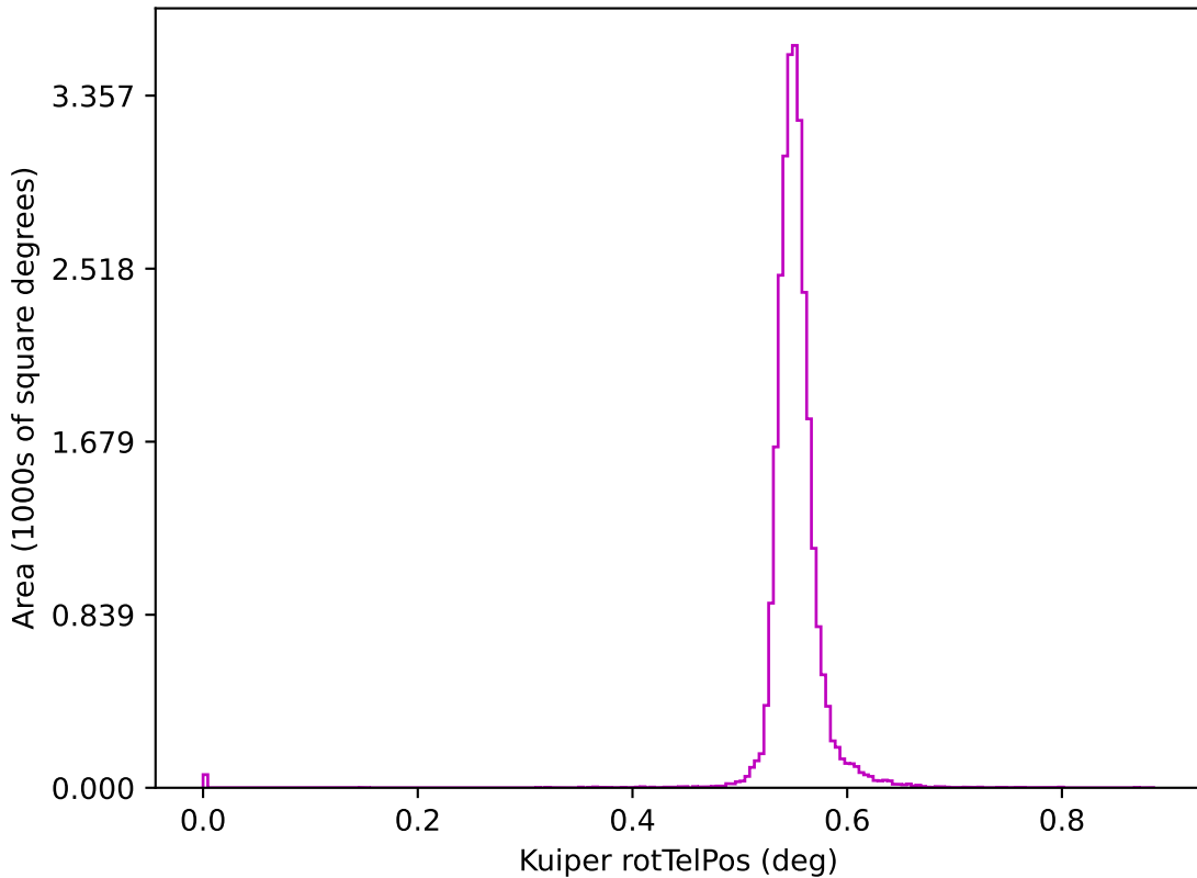
too_elab_r256_d2_giz_v3.4_10yrs z: Kuiper rotTelPos
