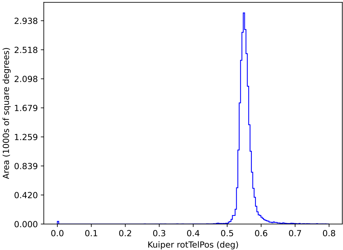
too_elab_r256_d2_giz_v3.4_10yrs y: Kuiper rotTelPos
