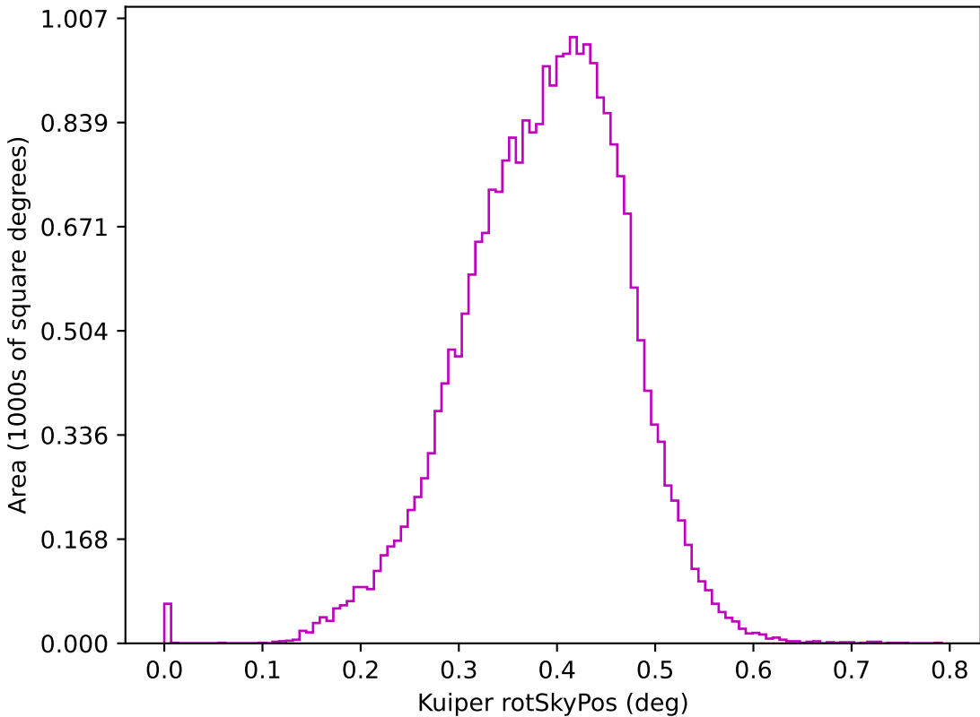
too_elab_r256_d2_giz_v3.4_10yrs z: Kuiper rotSkyPos
