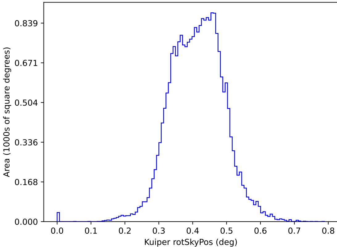
too_elab_r256_d2_giz_v3.4_10yrs y: Kuiper rotSkyPos
