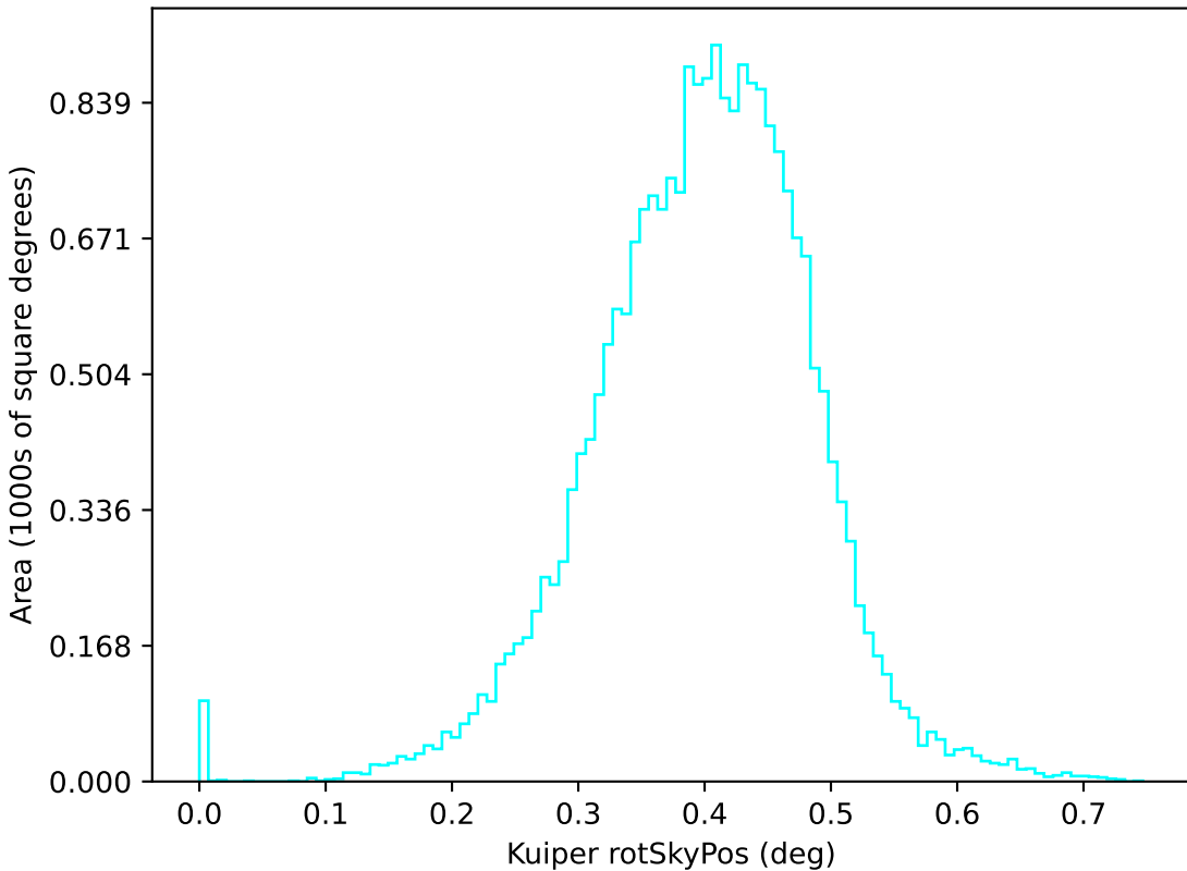
too_elab_r256_d2_giz_v3.4_10yrs u: Kuiper rotSkyPos
