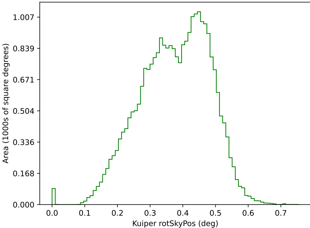
too_elab_r256_d2_giz_v3.4_10yrs g: Kuiper rotSkyPos
