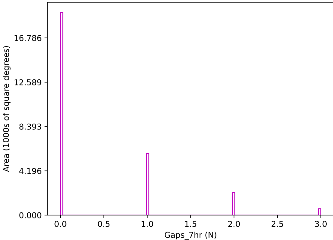
too_elab_r256_d2_giz_v3.4_10yrs z band: Gaps_7hr
