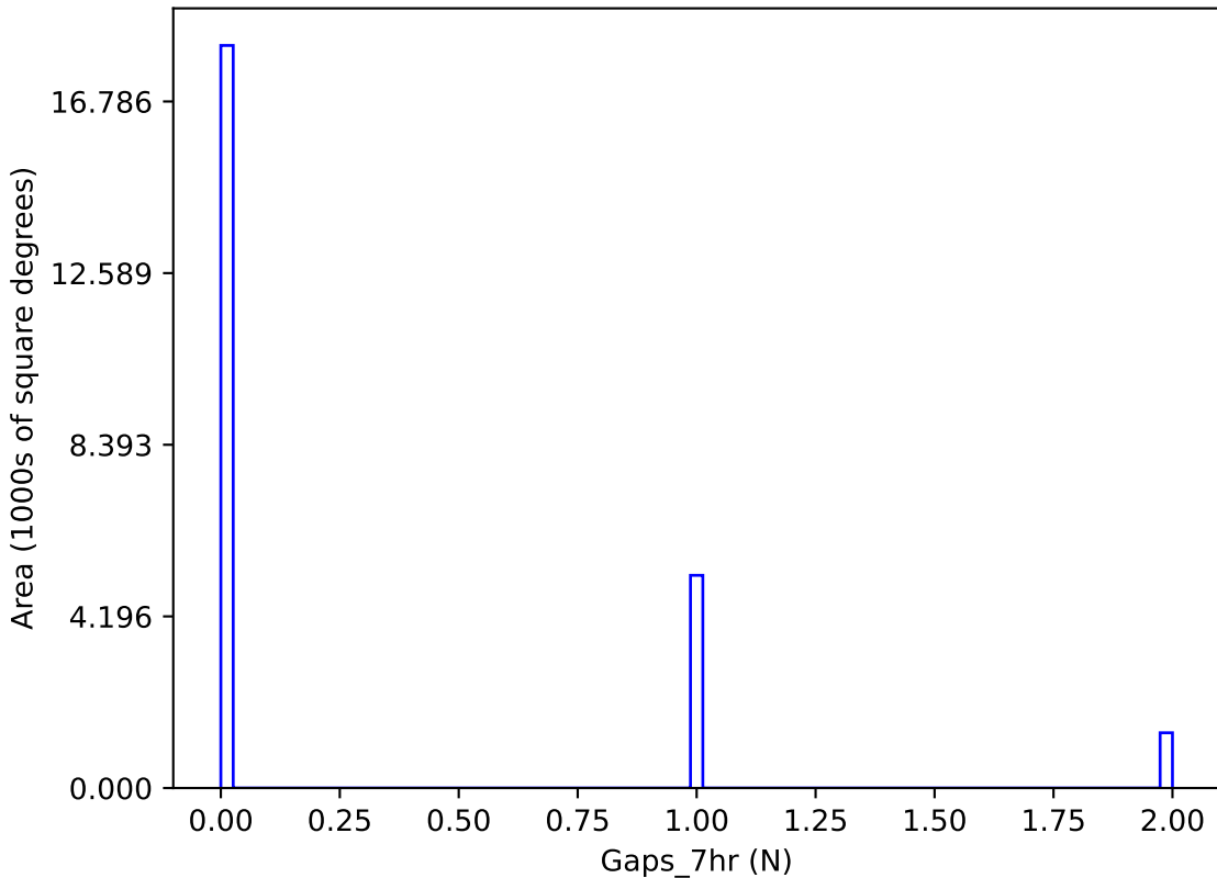
too_elab_r256_d2_giz_v3.4_10yrs y band: Gaps_7hr
