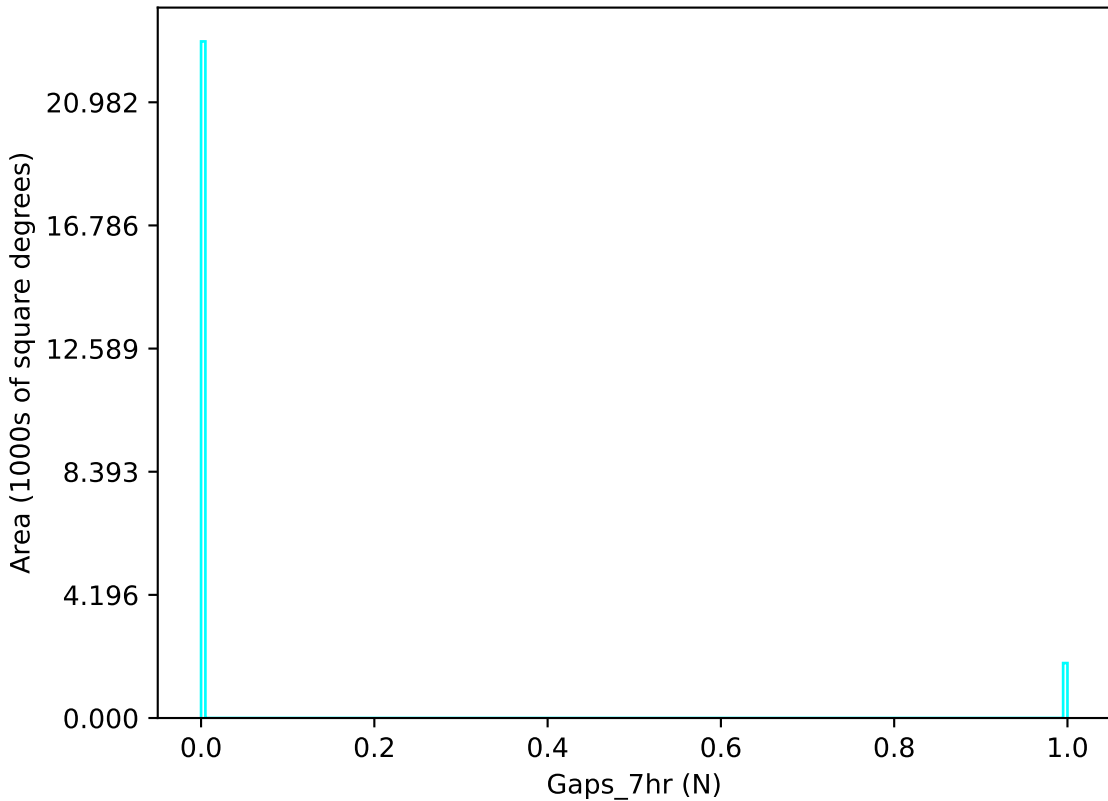
too_elab_r256_d2_giz_v3.4_10yrs u band: Gaps_7hr
