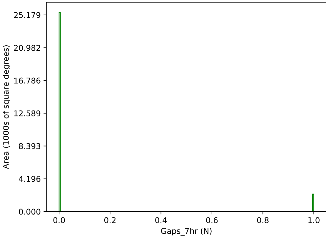
too_elab_r256_d2_giz_v3.4_10yrs g band: Gaps_7hr
