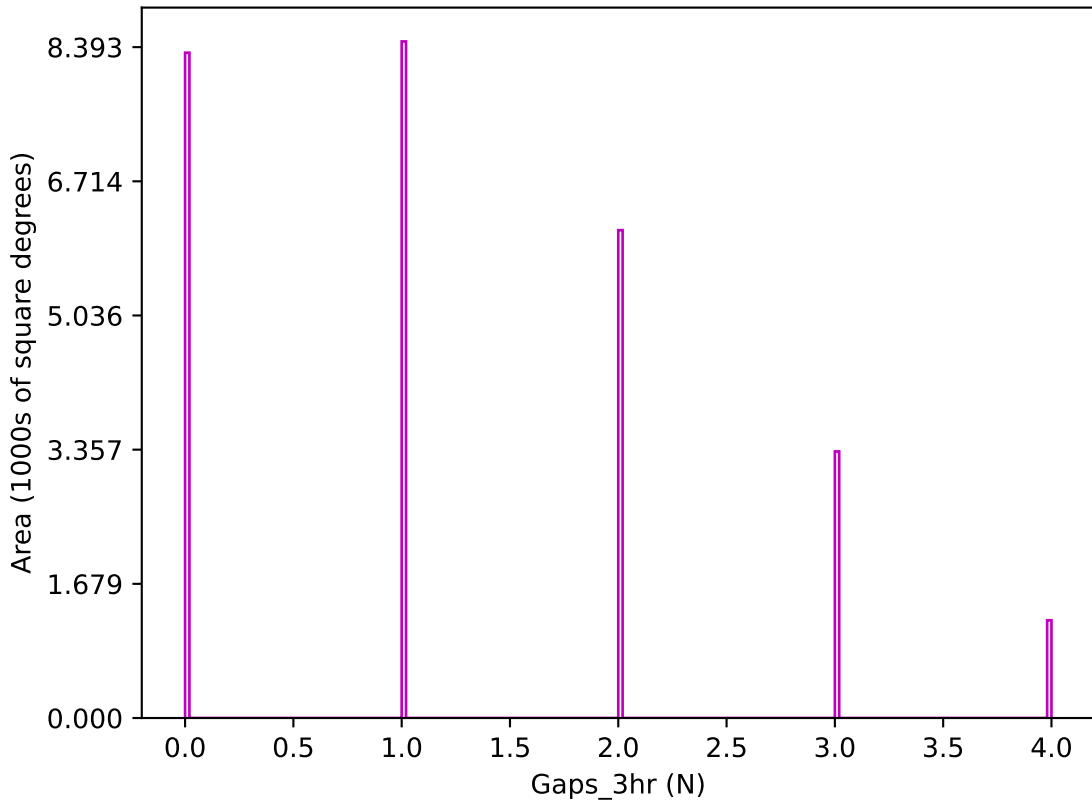
too_elab_r256_d2_giz_v3.4_10yrs z band: Gaps_3hr
