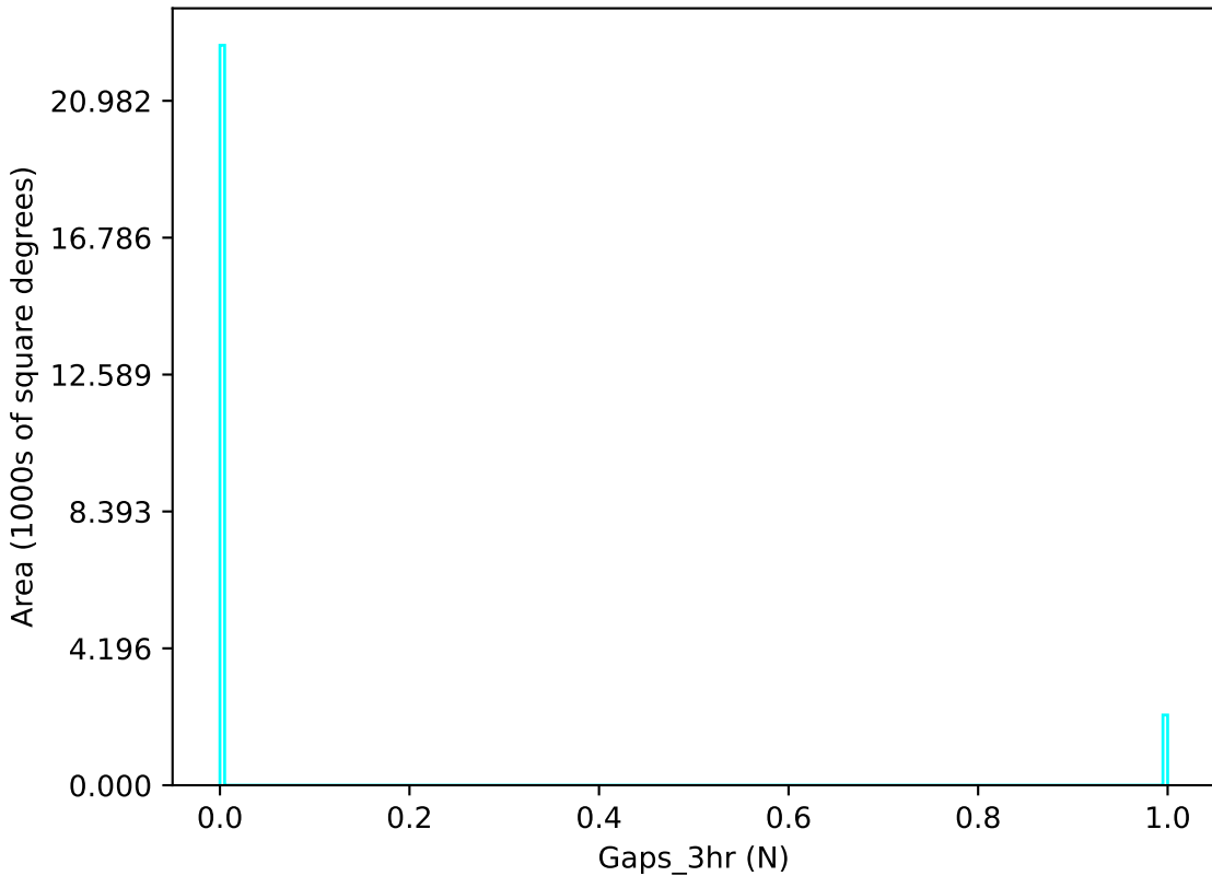
too_elab_r256_d2_giz_v3.4_10yrs u band: Gaps_3hr
