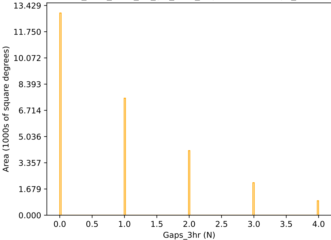
too_elab_r256_d2_giz_v3.4_10yrs r band: Gaps_3hr
