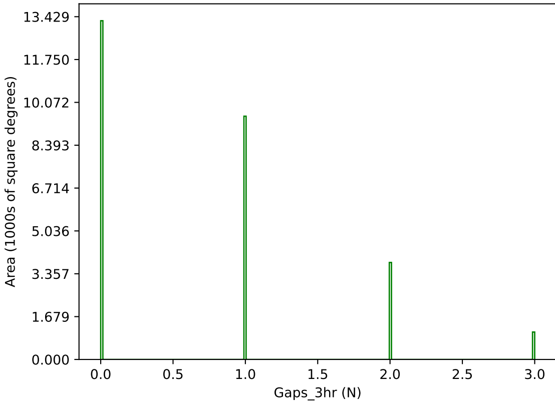
too_elab_r256_d2_giz_v3.4_10yrs g band: Gaps_3hr
