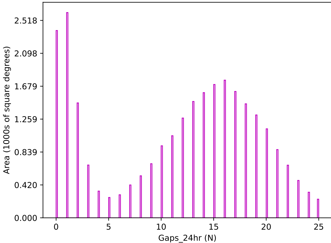
too_elab_r256_d2_giz_v3.4_10yrs z band: Gaps_24hr
