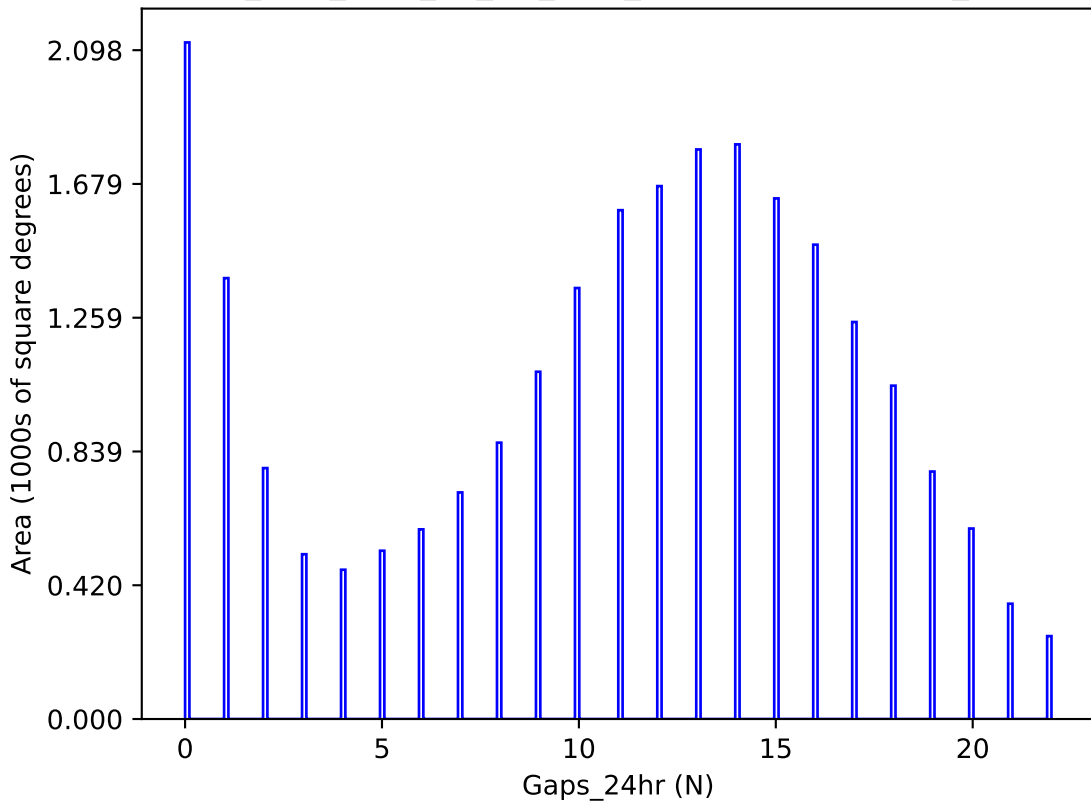
too_elab_r256_d2_giz_v3.4_10yrs y band: Gaps_24hr
