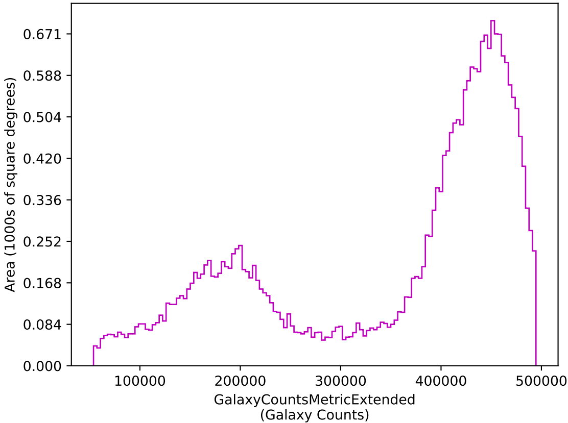
too_elab_r256_d2_giz_v3.4_10yrs z: GalaxyCountsMetricExtended
