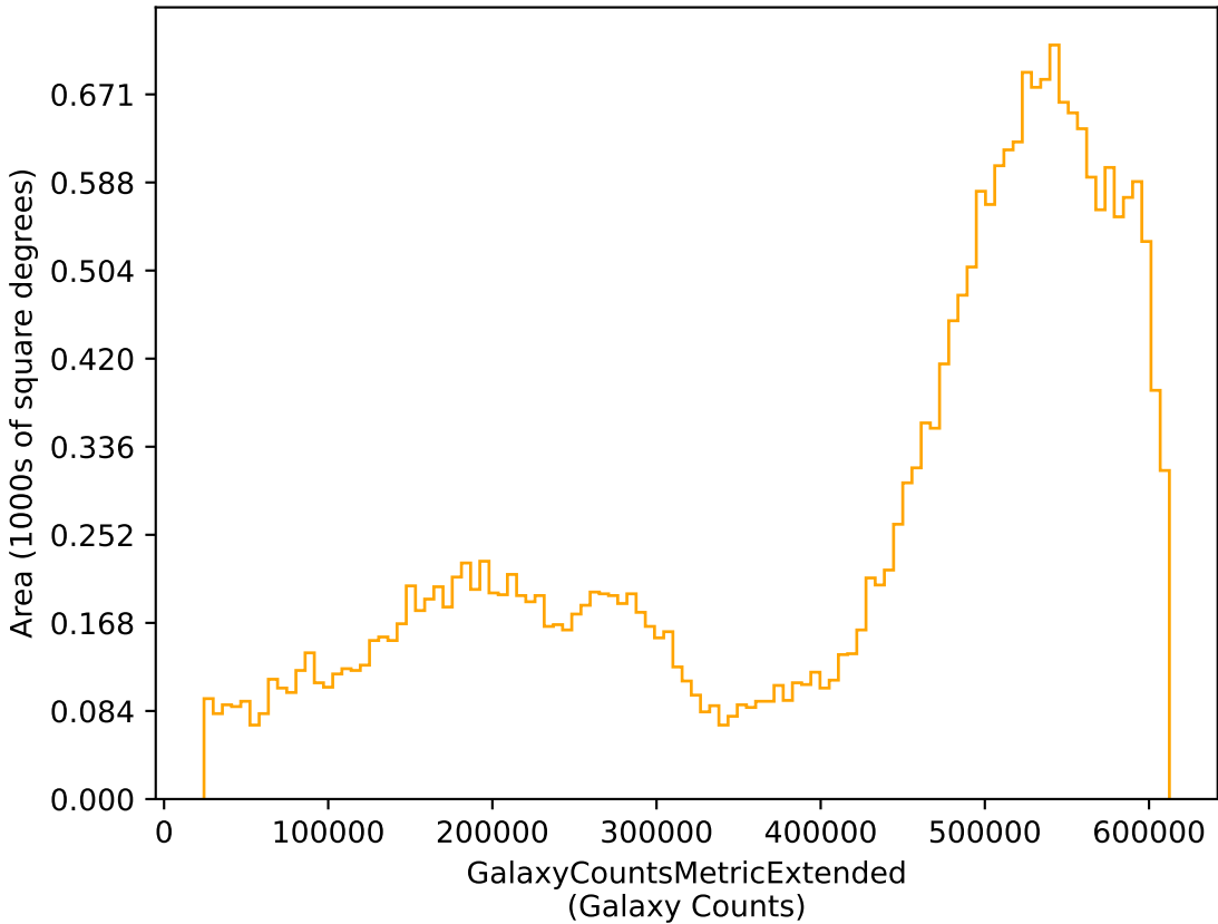
too_elab_r256_d2_giz_v3.4_10yrs r: GalaxyCountsMetricExtended
