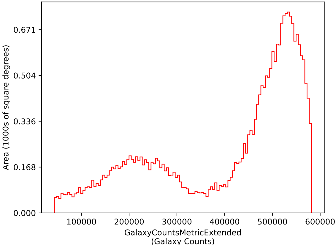
too_elab_r256_d2_giz_v3.4_10yrs i: GalaxyCountsMetricExtended
