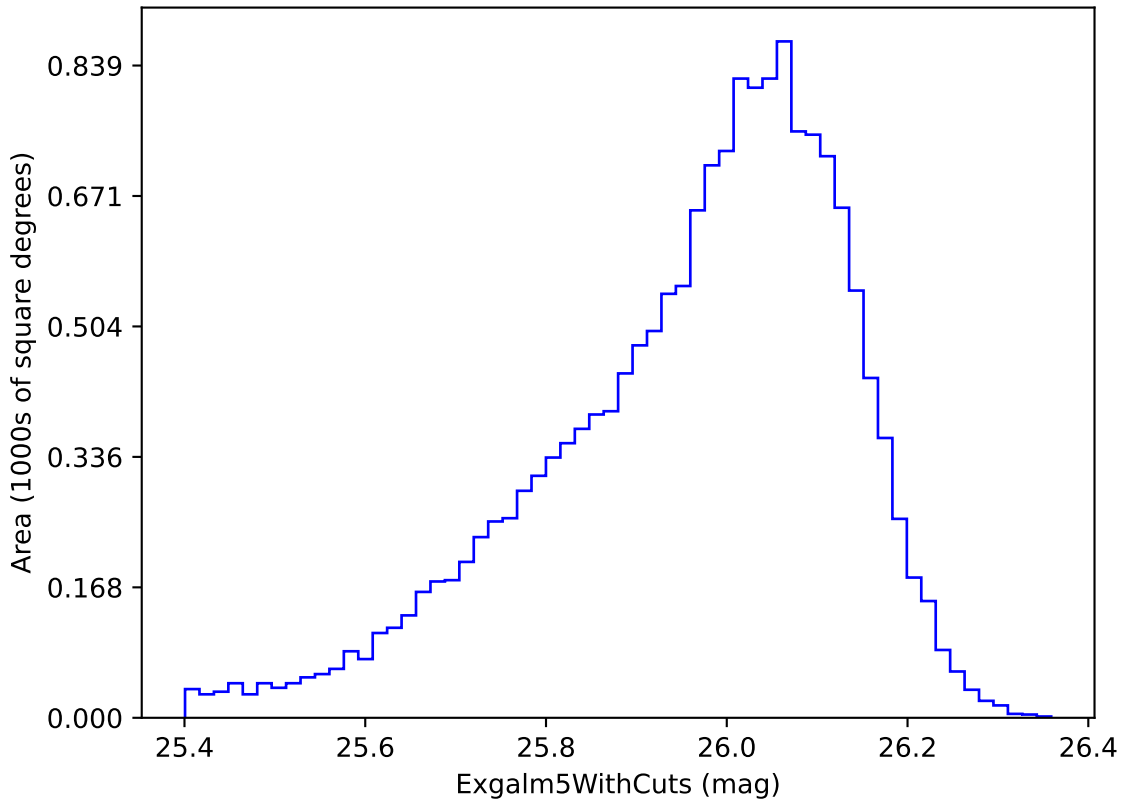
too_elab_r256_d2_giz_v3.4_10yrs i band non-DD year 4: Exgal5WithCuts
