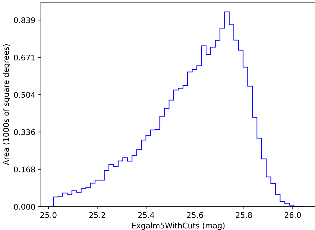
too_elab_r256_d2_giz_v3.4_10yrs i band non-DD year 2: ExgalM5WithCuts
