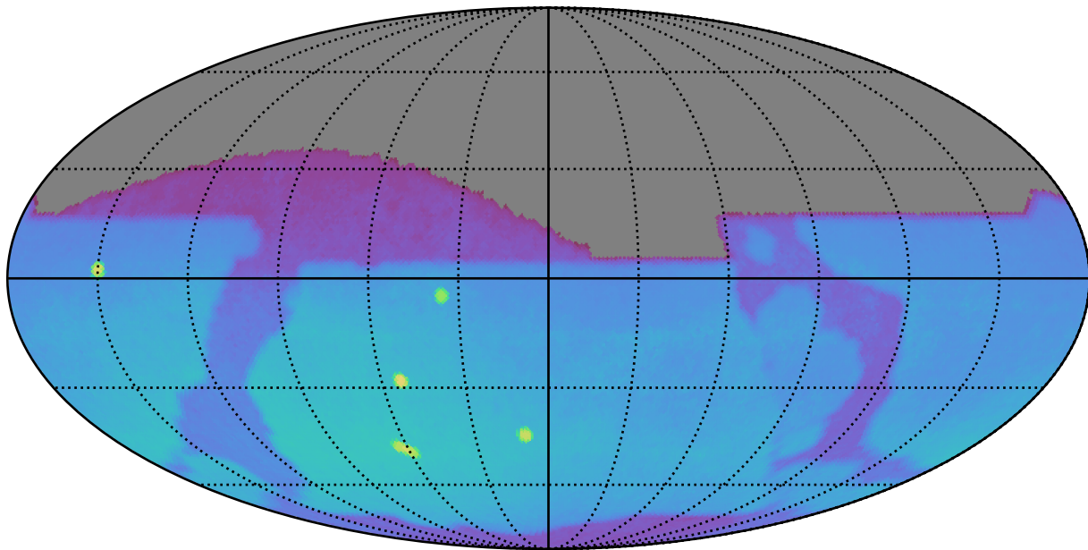
too_elab_r256_d2_giz_v3.4_10yrs : Brown Dwarf, L7
