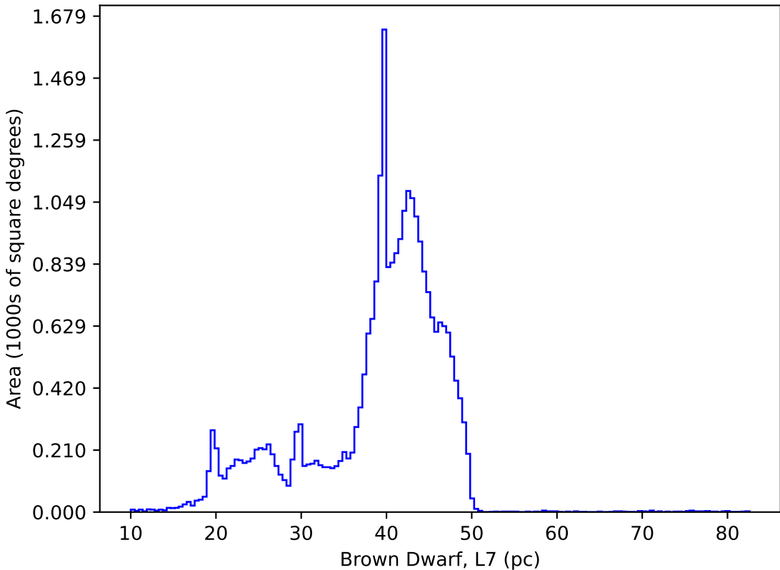
too_elab_r256_d2_giz_v3.4_10yrs : Brown Dwarf, L7
