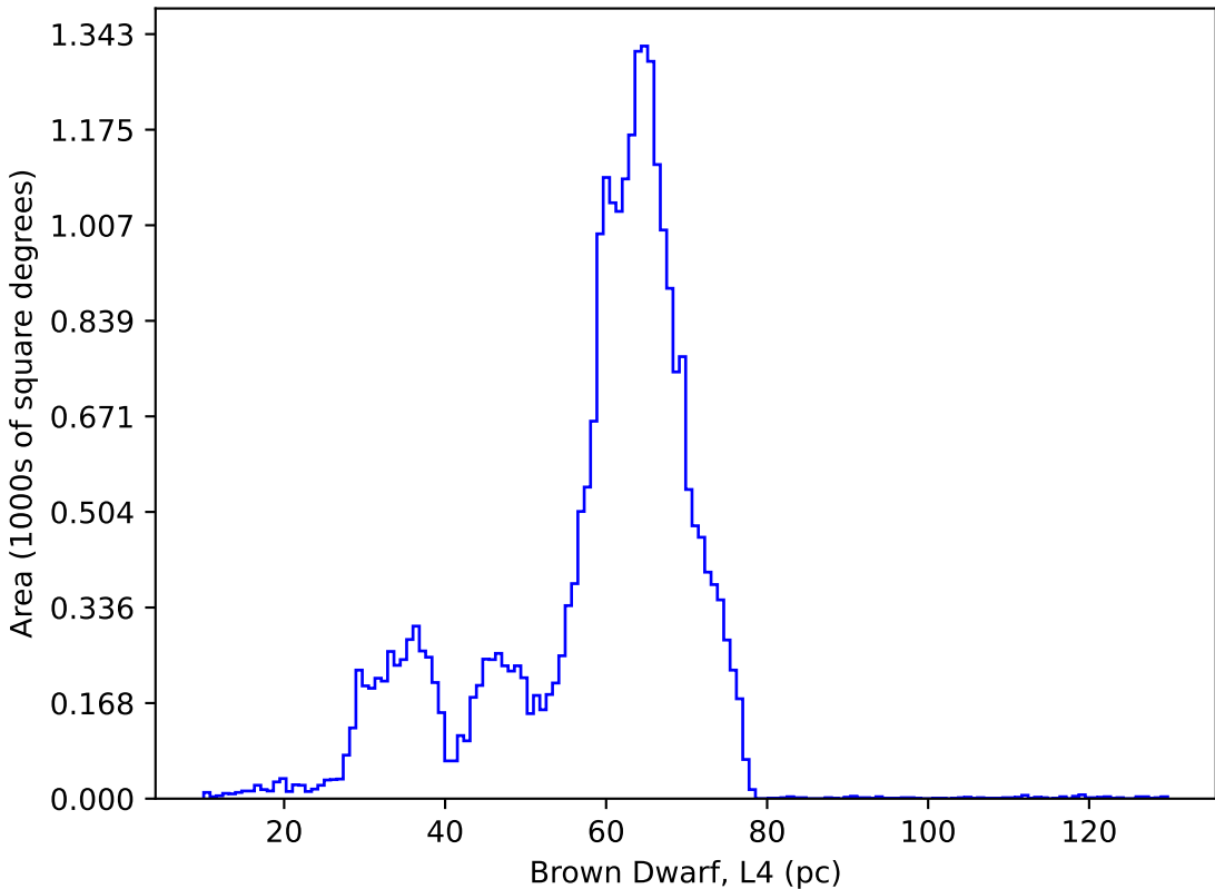
too_elab_r256_d2_giz_v3.4_10yrs : Brown Dwarf, L4
