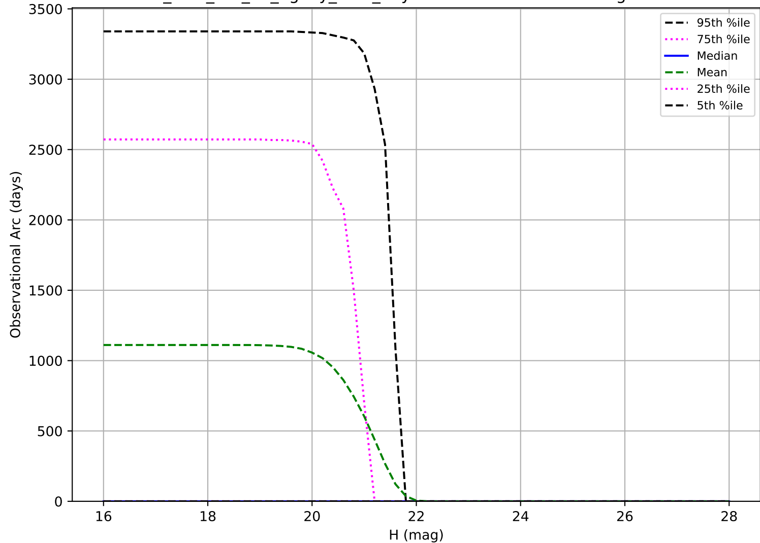
too_elab_r16_d3_ugrizy_v3.4_10yrs: Observational Arc Length Vatra
