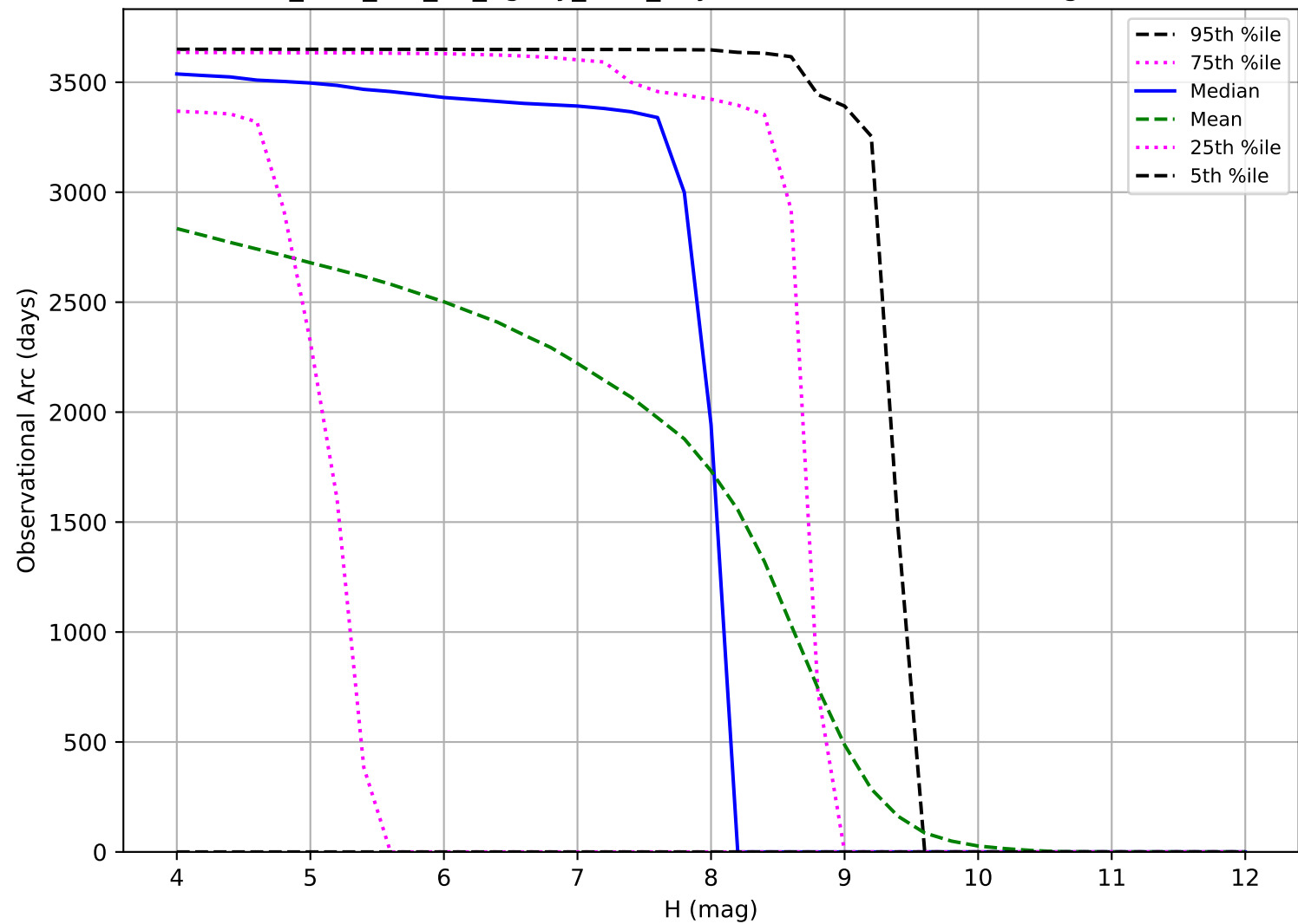
too_elab_r16_d3_ugrizy_v3.4_10yrs: Observational Arc Length TNO
