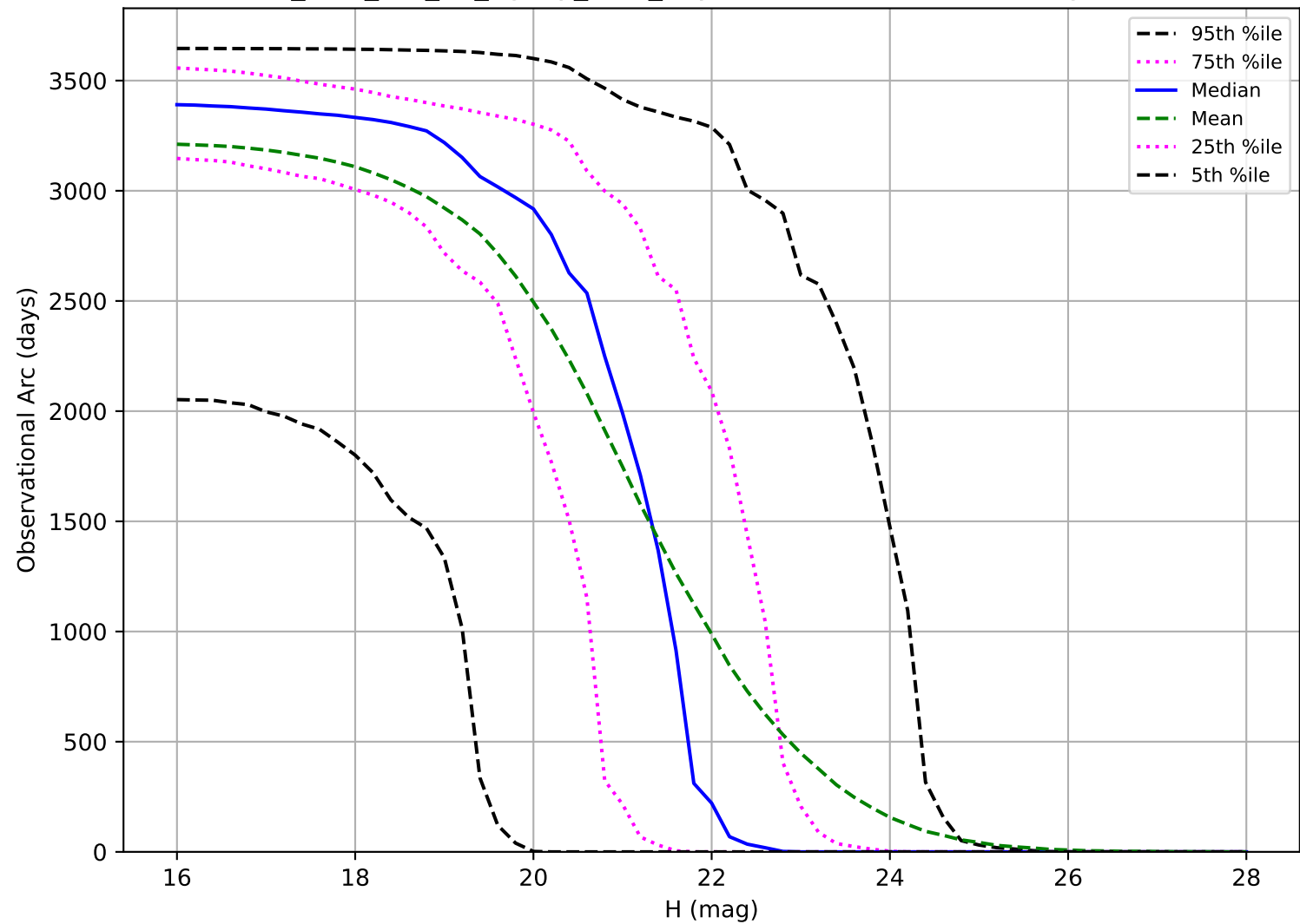
too_elab_r16_d3_ugrizy_v3.4_10yrs: Observational Arc Length PHA
