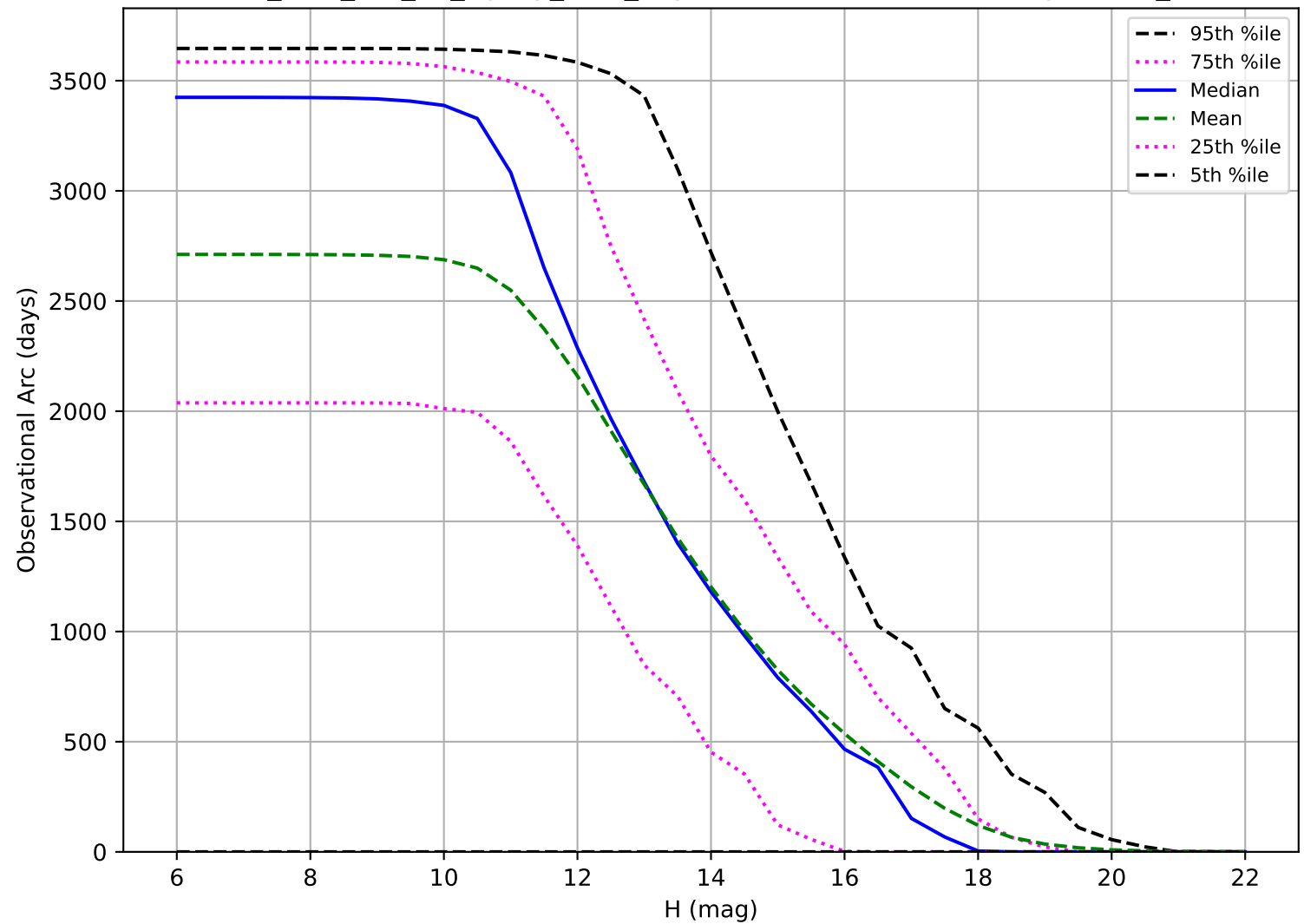
too_elab_r16_d3_ugrizy_v3.4_10yrs: Observational Arc Length OCC_r5
